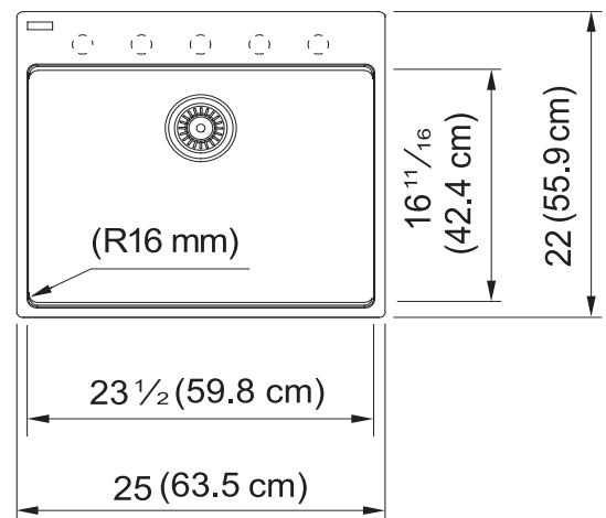
Dimensional Drawing
