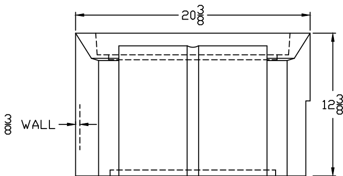
DFW39C-12-BODY
