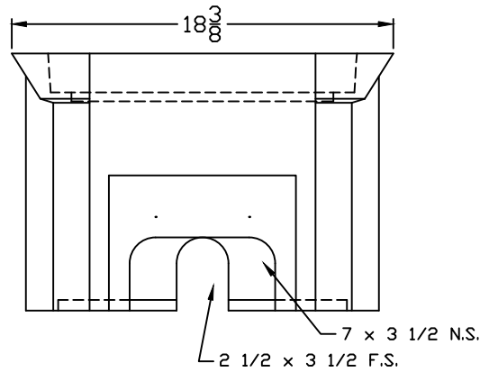
DFW39C-12-1
